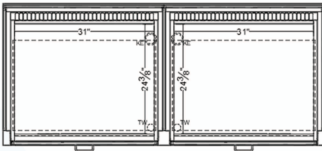
(floor plan)
